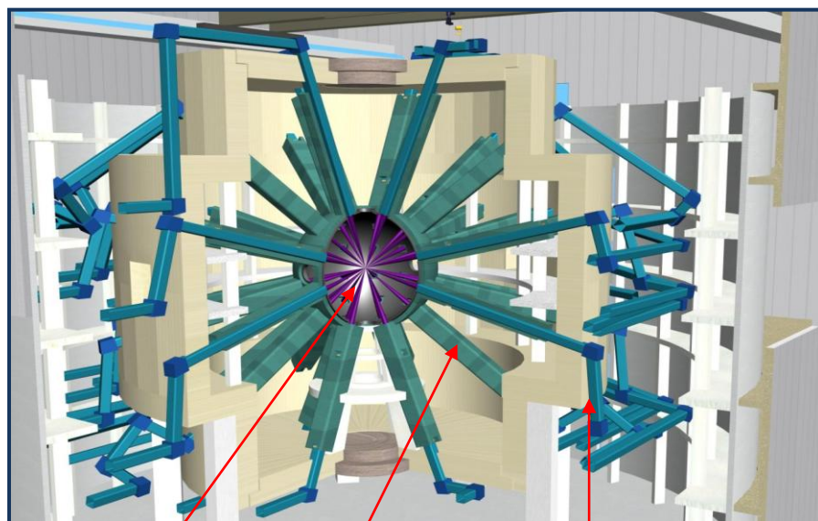
Target Chamber Target Area Concrete Bioshield
